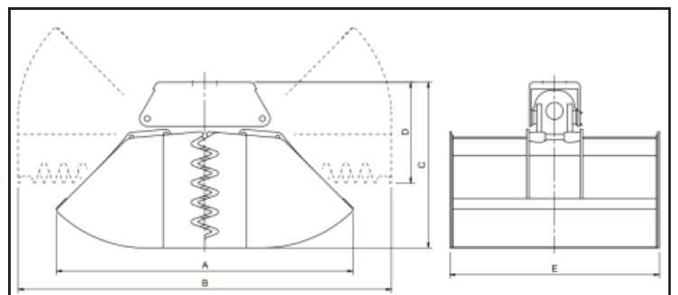
HEMA Wood Chip Grapple FG90-3000
