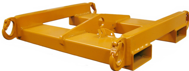
1,6 tons Big Bag Yoke for Truck or crane hook.
