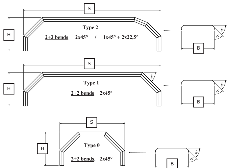
Mudguard with bent edges.
