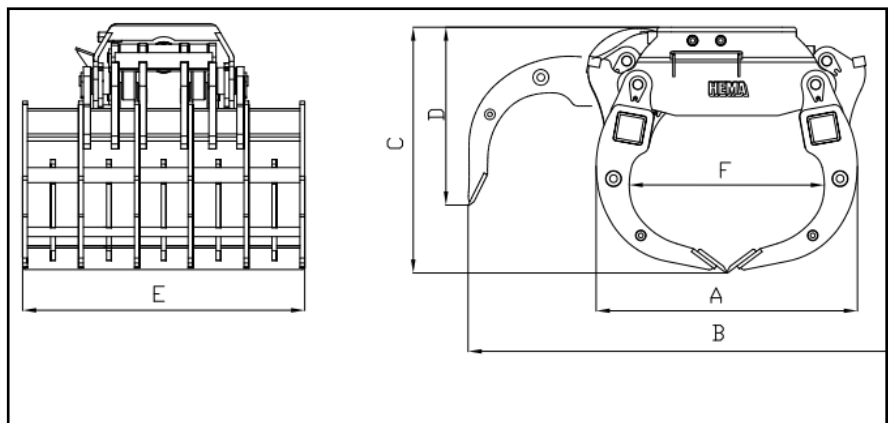
HEMA Waste Grapple AGX-T 60/100-1400
