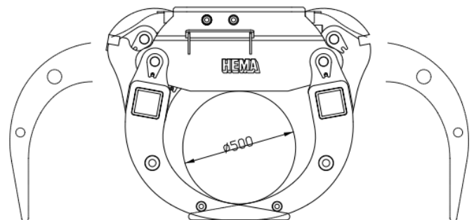
HEMA Waste Grapple AGX-T 60/100-1400
