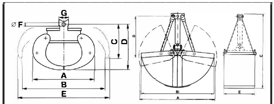
Orange Peel Grapple PFO-5/100
