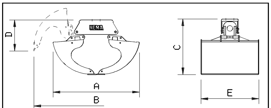
50-90 Combi Grapple with side plates
